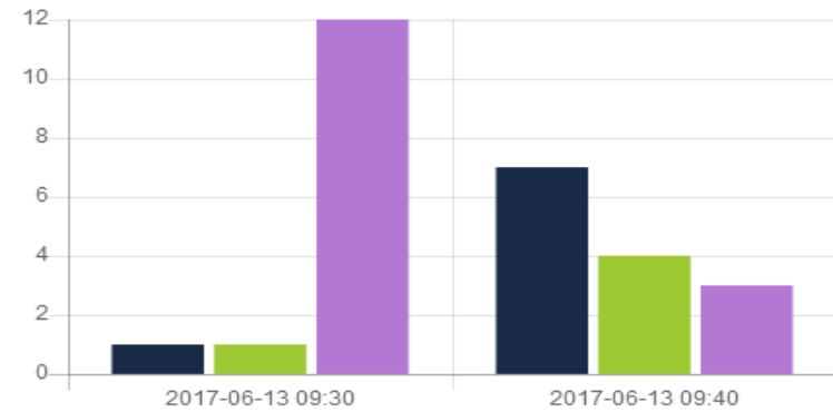
Logical Poll
