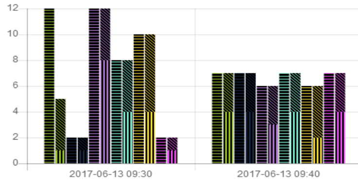
Managers
